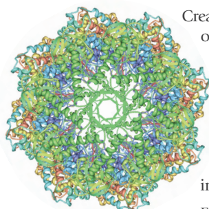
Image of 3izi 4 created using Protein Workshop
